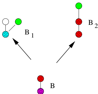
Figure 6: Illustrating Bell causality - spectators do not affect relative probability
