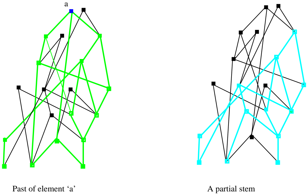
Figure 2: An example of a ('typical?') 20 element causal set
